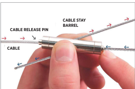
FIGURE 4 Cable Stay Operation
