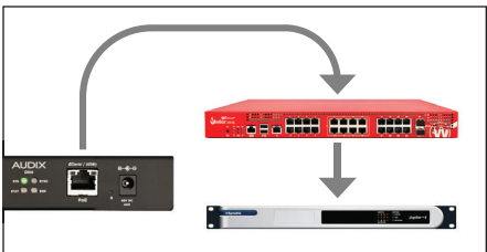
FIGURE 6 Connect the DN4 Dante interface to a PoE switch (see DN4 guide).
